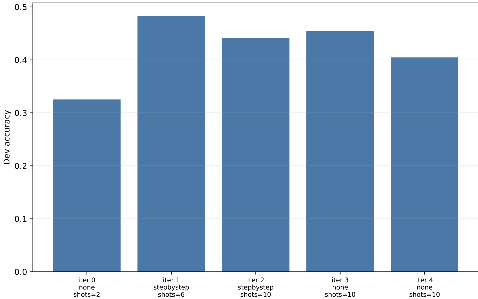
Prompt/Strategy Diversity Summary
